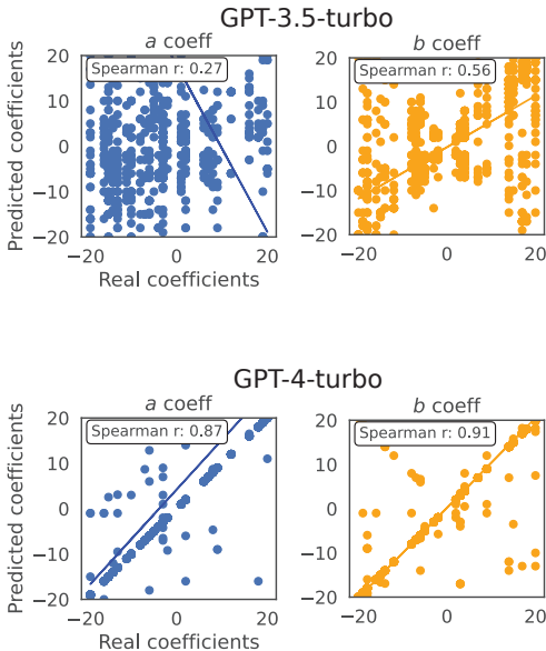
Figure 2: Real coefficients of linear functions and relationship to hypothesized coefficients for GPT-3.5-turbo and GPT-4-turbo. Remaining models can be found in Appendix D. The x-axis has been truncated for visualization purposes (as there are some large outlier hypotheses). GPT-4-turbo is able to induce a reasonable function in-context, but other models struggle.
